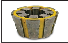
T400 14.2mm Die Set P/N:PF402-14.2D
